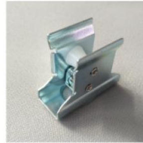
35mm Locker 35mm锁具
